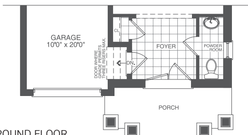
GROUND FLOOR ELEVATION B 1869 sf
