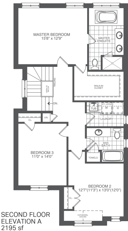
OPTIONAL SECOND FLOOR ELEVATION A 2195 sf
