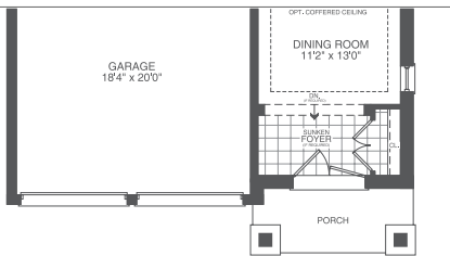
GROUND FLOOR ELEVATION B 2334 sf
