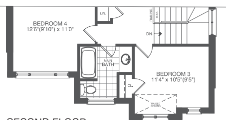
SECOND FLOOR ELEVATION C 2316/2314 sf
