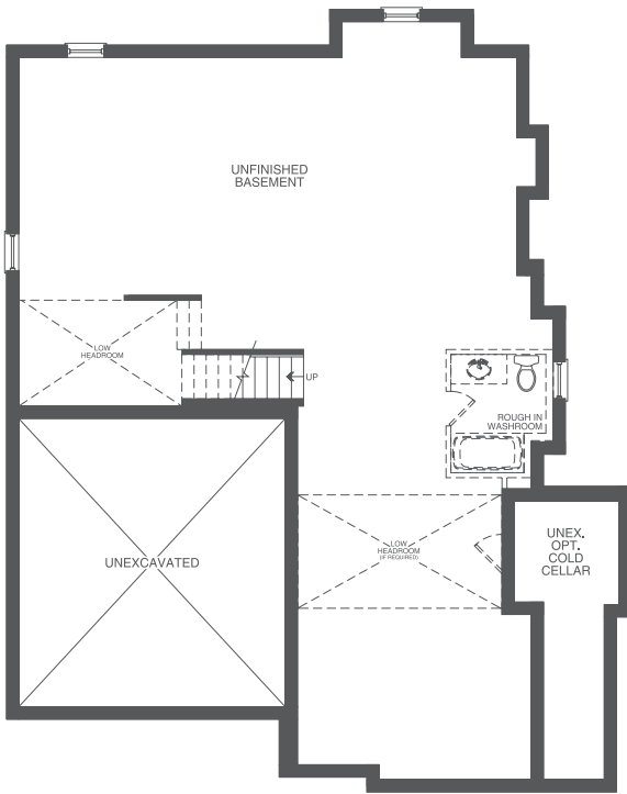
UNFINISHED BASEMENT ELEVATION B 3066 sf
