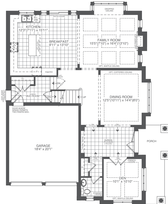
GROUND FLOOR ELEVATION B 3066 sf
