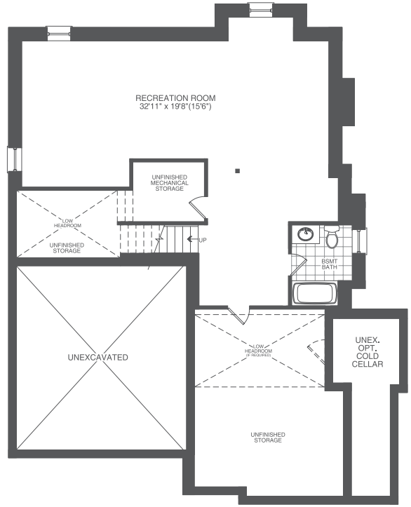
856 sf OF OPT. FINISHED BASEMENT ELEVATION B 3922 sf
