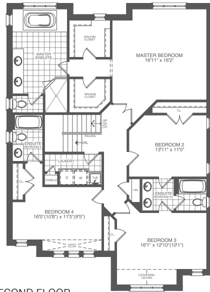
SECOND FLOOR ELEVATION A 3102 sf
