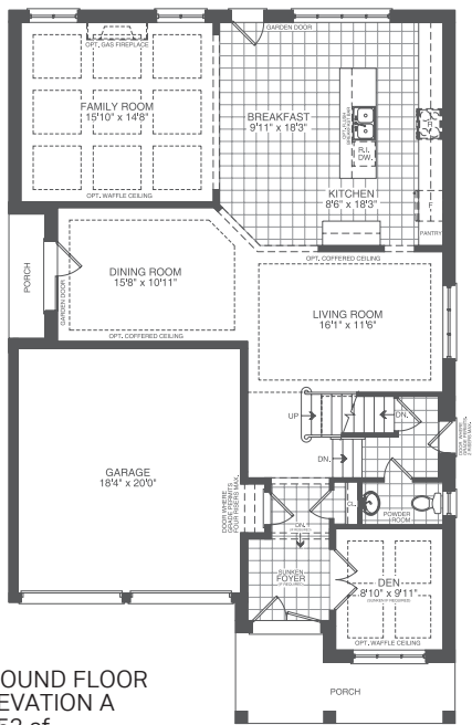
ELEVATION A 3,253 sq. ft.
