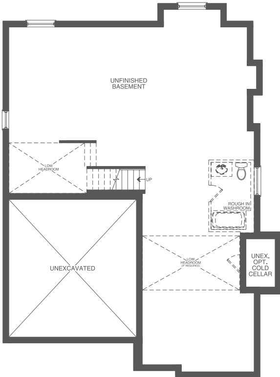
UNFINISHED BASEMENT ELEVATION C 3034 sf
