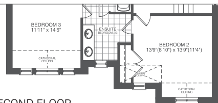
SECOND FLOOR ELEVATION B 3259 sf
